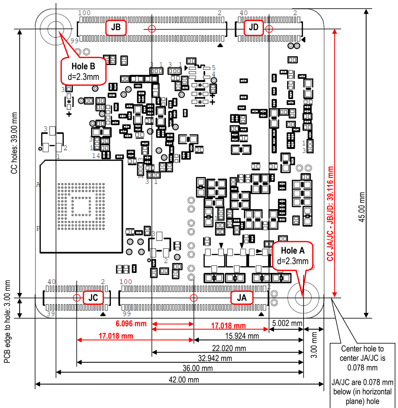
Figure 10 – iMX7ULP uCOM Board Mechanical Outline, View from Bottom Side
