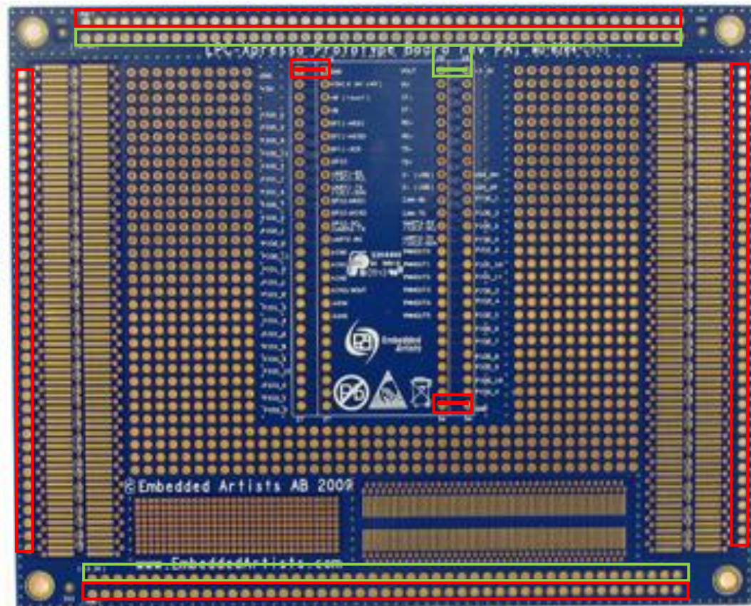
Figure 6 – Board Powering
