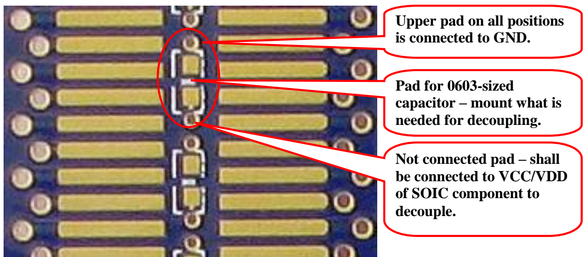
Figure 12 – 0603 pads in SOIC Area
