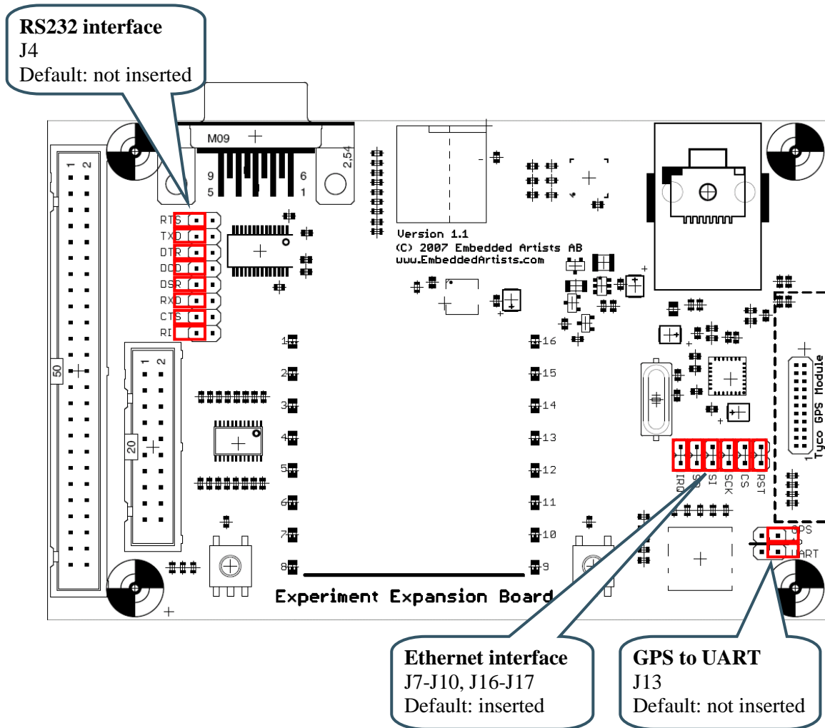
Figure 1 – Experiment Expansion Board Jumpers
