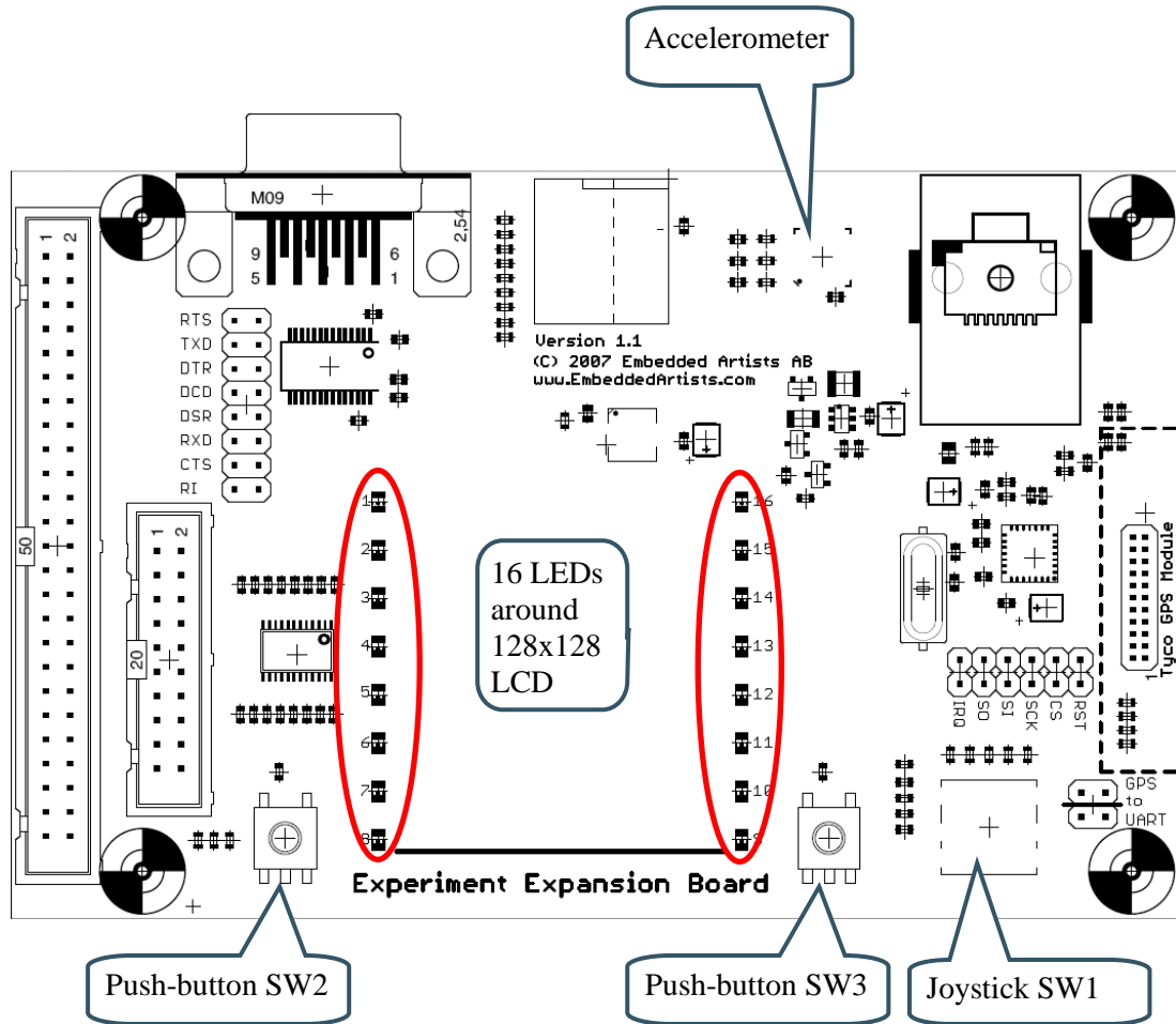
Figure 3 - Experiment Expansion Board Important Components
