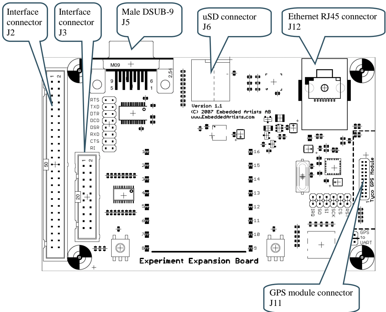
Figure 2 - Experiment Expansion Board External Connectors
